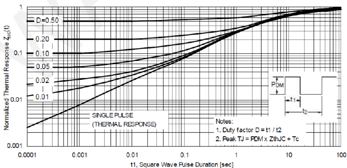
Figure 11 Maximum Transient Thermal Impedance WAN SEMICONDUCTOR (NINGBO) CO.,LTD
