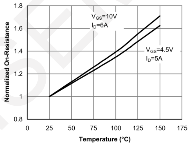
Rdson-Junction Temperature
