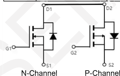
Schematic Diagram
