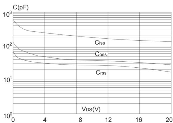
Capacitance Characteristics
