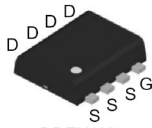
PDFN3X3 Pin Description
