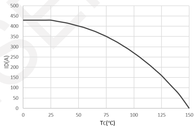
Current De-rating
