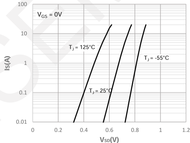
Body-Diode Characteristics
