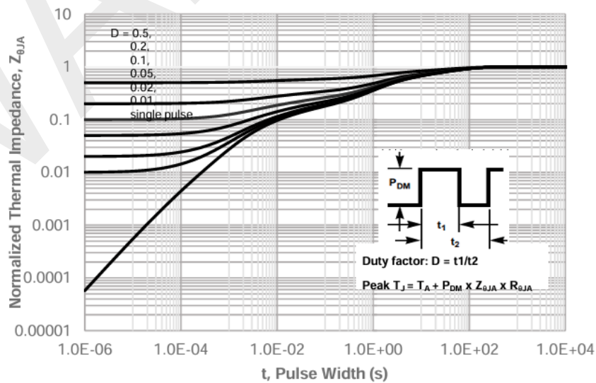
Normalized Maximum Transient Thermal Impedance
