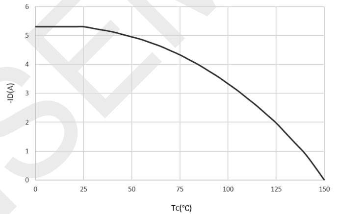
Current De-rating
