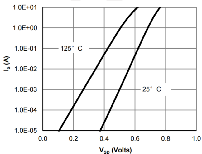
Body-diode Characteristics
