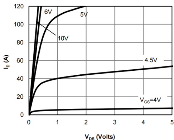
Saturation Characteristics
