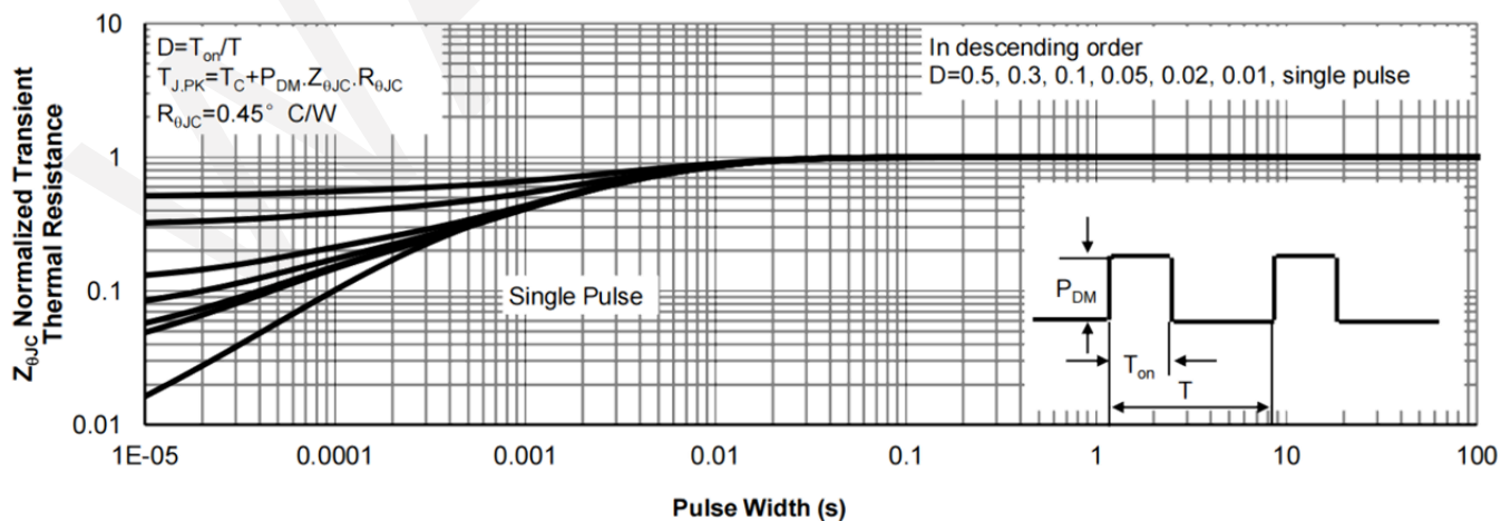
Maximum Transient Thermal Impedance
