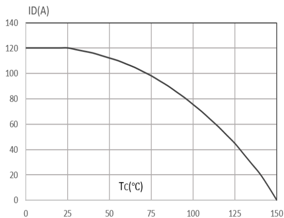
Current De-Rating
