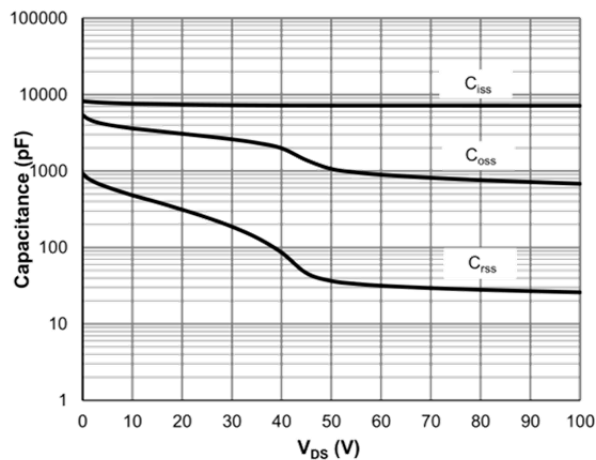
Capacitance Characteristics
