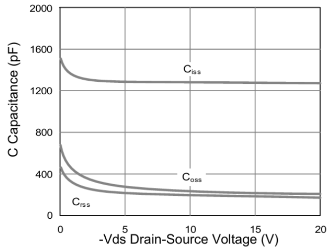
Capacitance Characteristics
