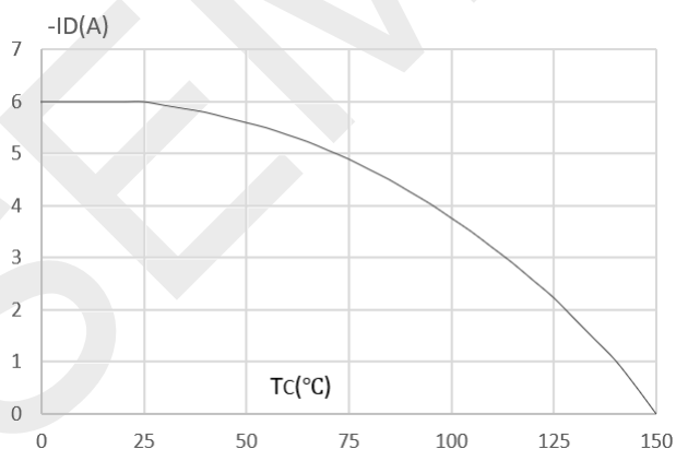
Current De-rating
