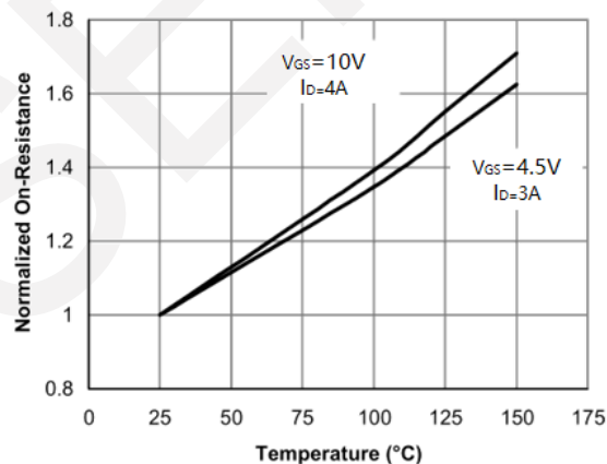
Drain-Source On-Resistance
