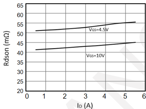
Drain-Source On-Resistance
