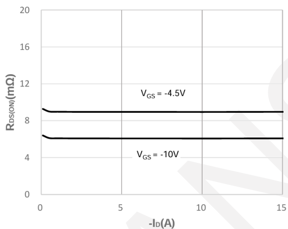
Rdson-Drain Current
