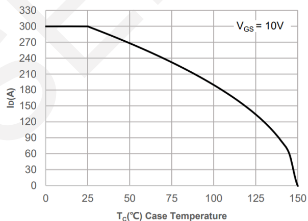
Current De-rating
