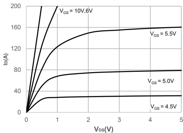
Saturation Characteristics
