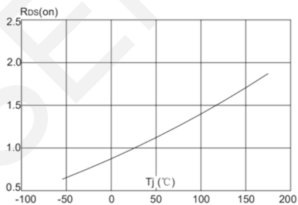
Rdson-Junction Temperature
