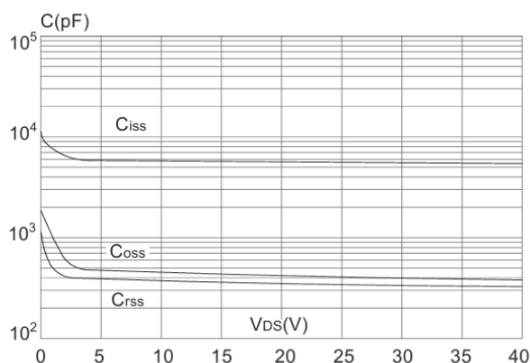
Capacitance Characteristics
