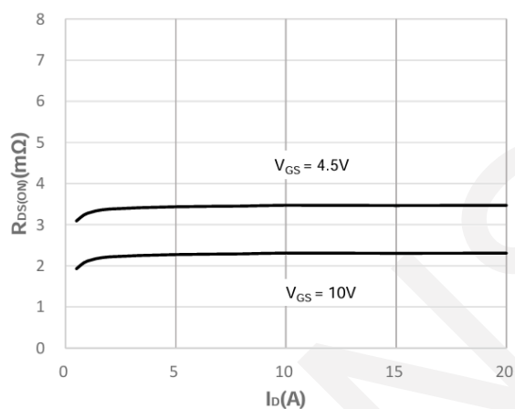
Rdson-Drain Current
