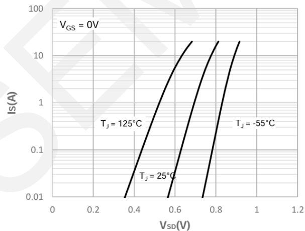
Body Diode Characteristic
