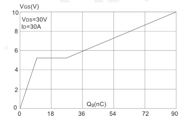
Gate Charge
