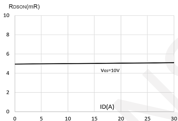
Rdson-Drain Current
