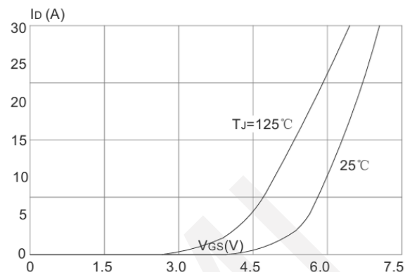
Transfer Characteristics
