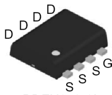
PDFN3x3-8L Pin Description
