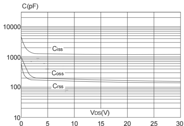
Capacitance Characteristics
