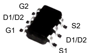
Pin Description
