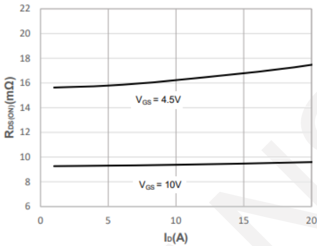
Rdson-Drain Current
