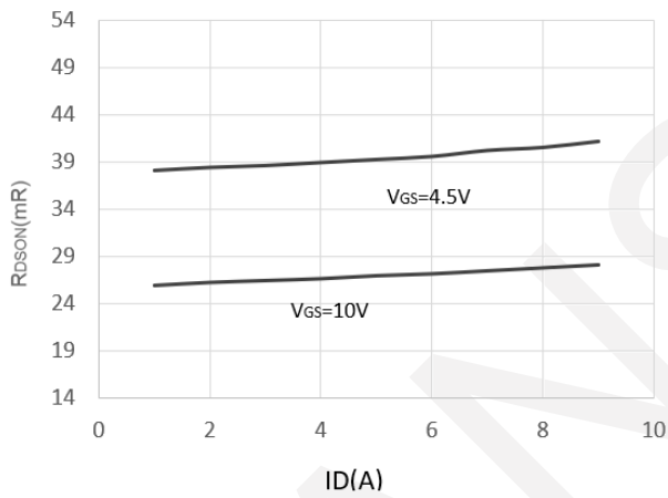
Drain-Source On-Resistance
