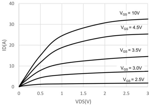
Output Characteristics
