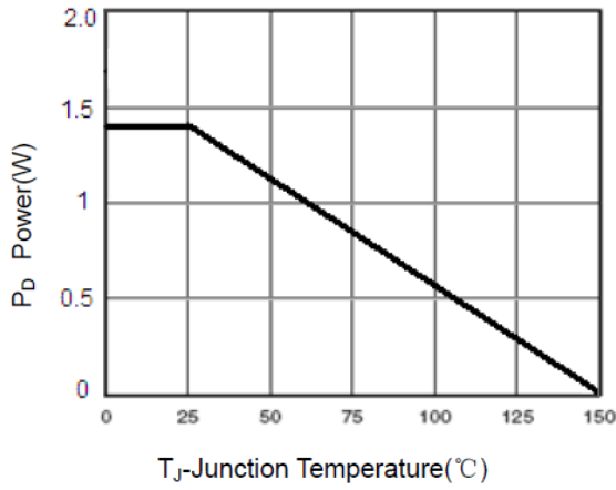
Power Dissipation
