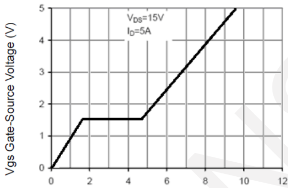
Gate Charge
