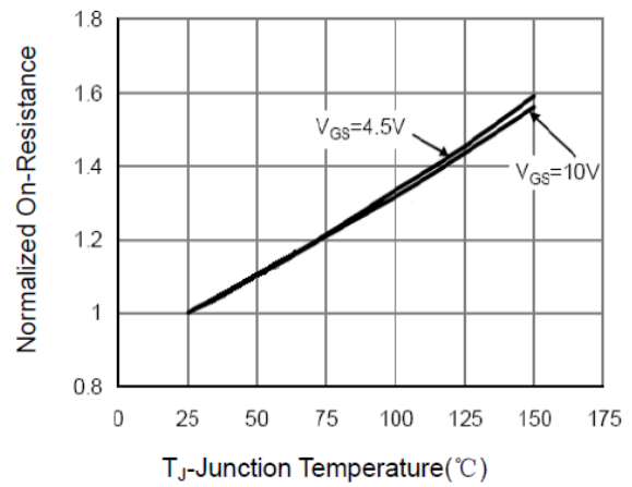
Drain-Source On-Resistance
