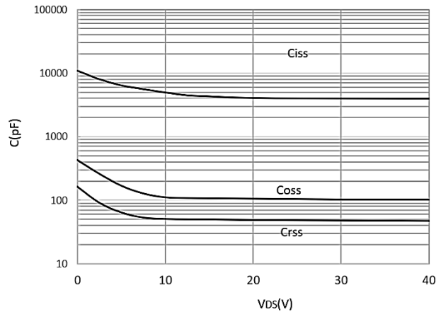
Capacitance Characteristics
