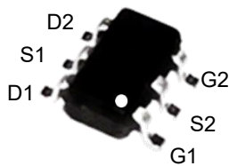
Pin Description
