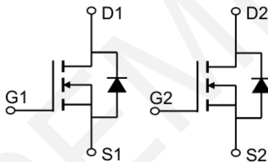
Schematic Diagram
