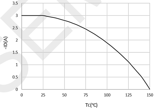
Current De-rating
