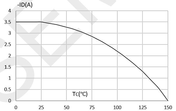
Current De-rating
