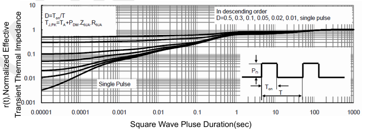
Maximum Effective Transient Thermal Impedance, Junction-to-Ambient
