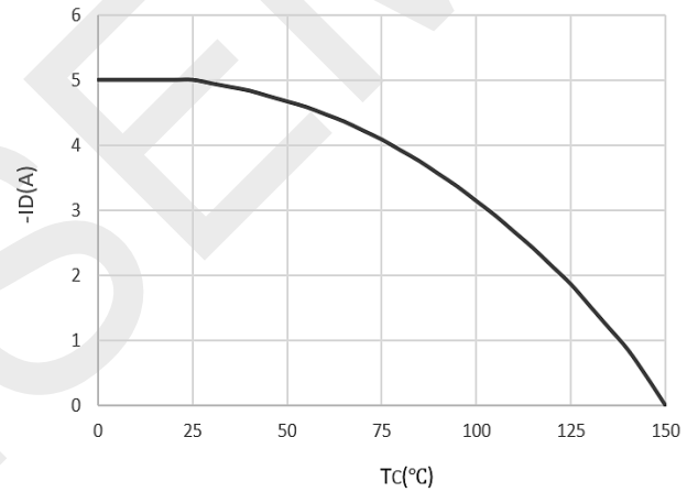
Current De-rating
