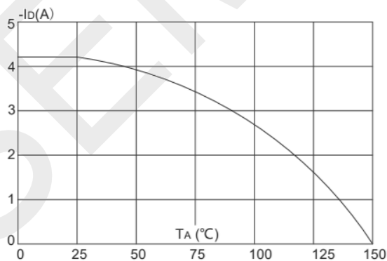
Current De-rating
