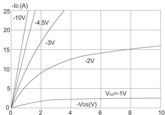
Output Characteristics
