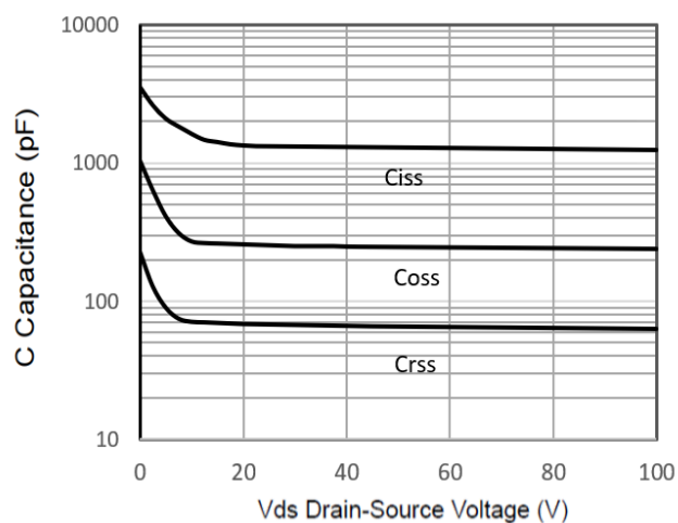
Capacitance Characteristics
