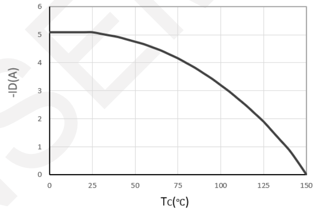
Maximum Continuous Drain Current vs. Case
