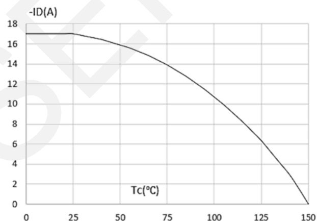
Maximum Continuous Drain Current vs. Case
