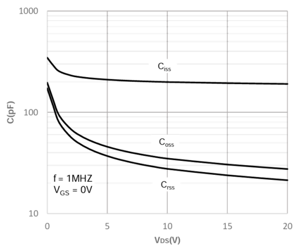
Capacitance Characteristics
