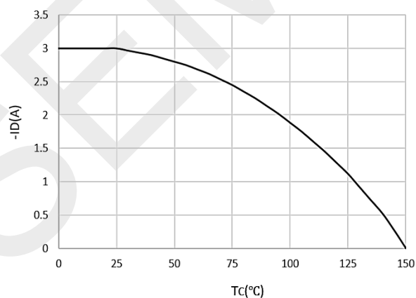
Current De-rating
