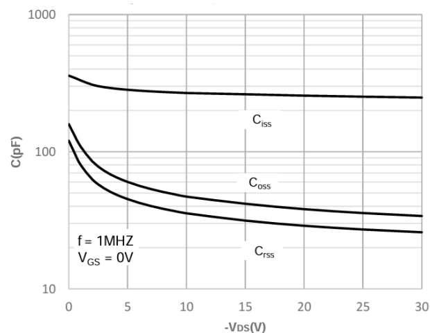
Capacitance Characteristics
