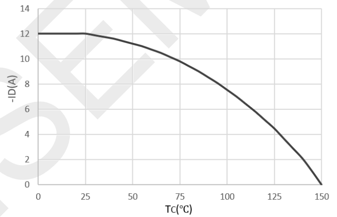
Current De-rating
