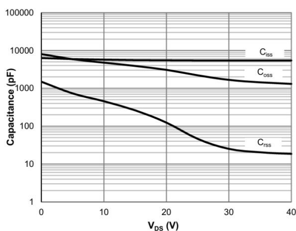
Capacitance Characteristics
