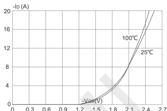
Transfer Characteristics
