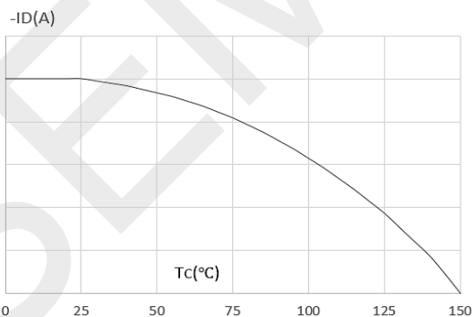
Maximum Continuous Drain Current vs. Case Temperature
