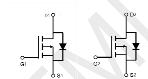
Schematic Diagram
